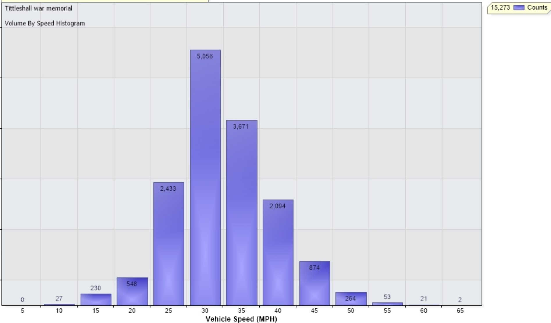
Vehicle Counts Vs. Speed [Tittleshall war memorial: Incoming]
