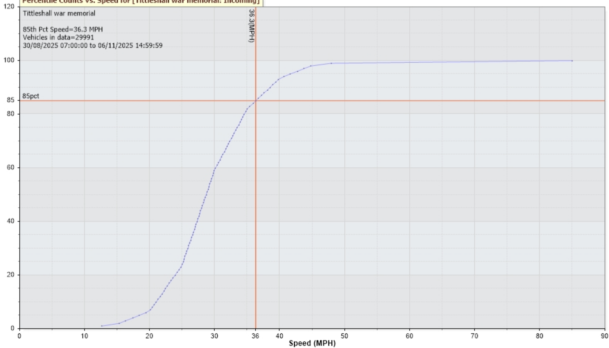
Percentile Counts Vs. Speed for [Tittleshall war memorial: Incoming]
