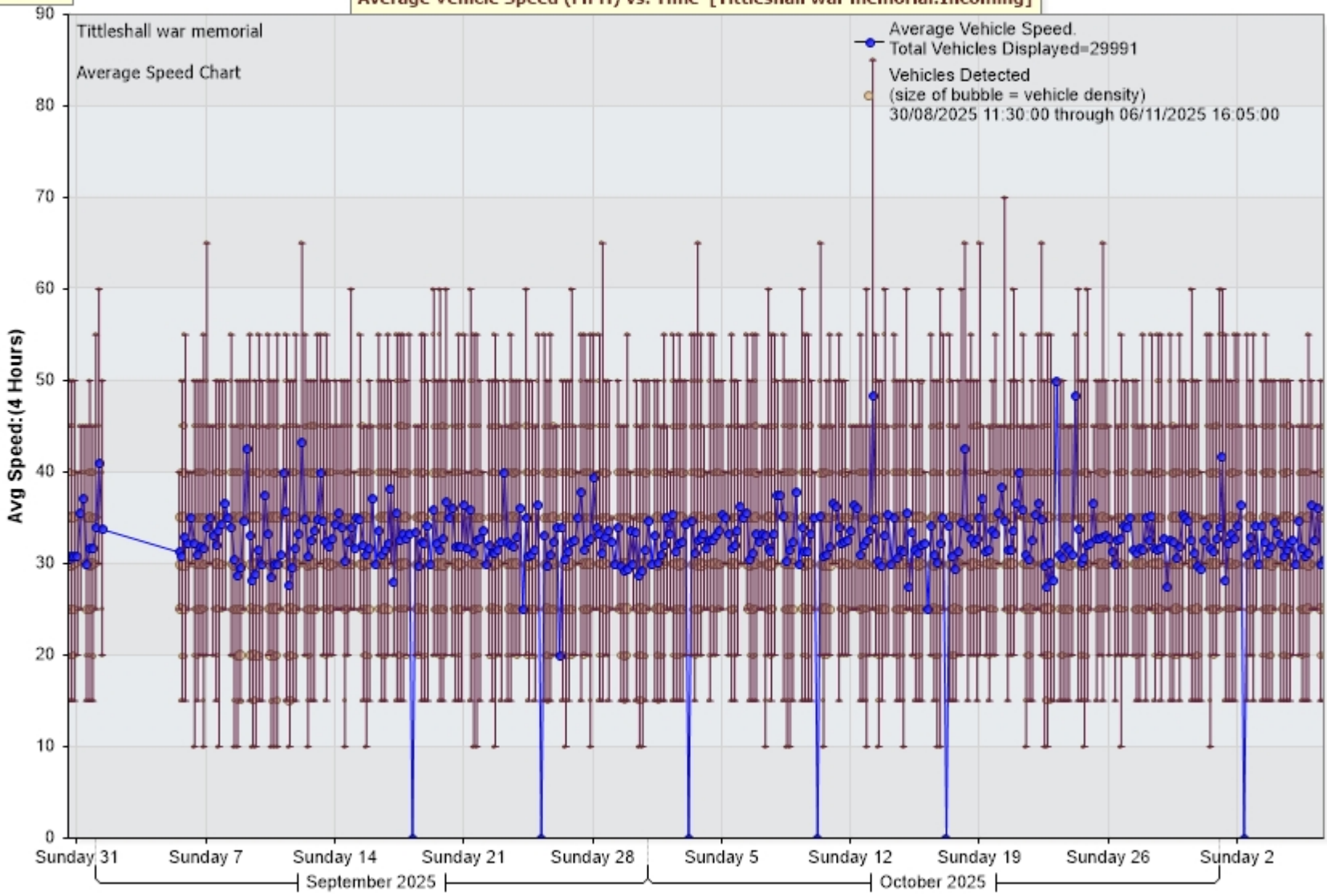
Average Vehicle Speed (MPH) vs. Time [Tittleshall war memorial:Incoming]
