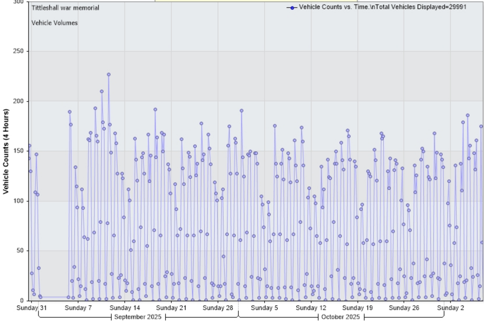
Vehicle Counts vs. Time [Tittleshall war memorial: Incoming]
